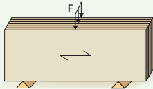
A f_{m,0,edge} and E_{0,edge} Edge-wise, parallel to grain*
