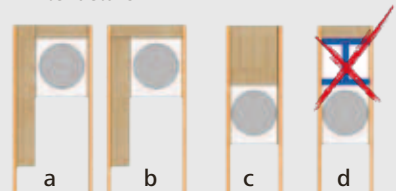
Lintel details
