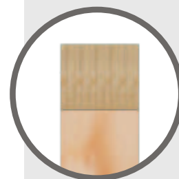
Glued multi-part STEICO LVL R lintel as continuous top plate
